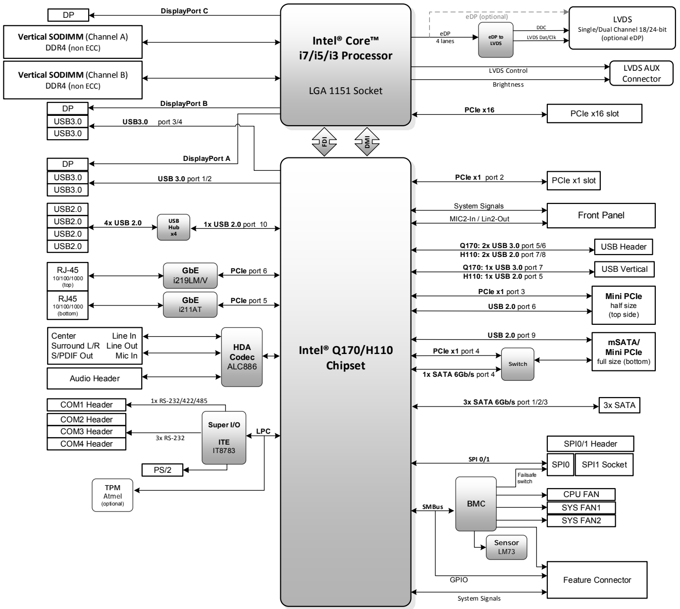
Figure 1: AmITX-SL-G Functional Block Diagram
