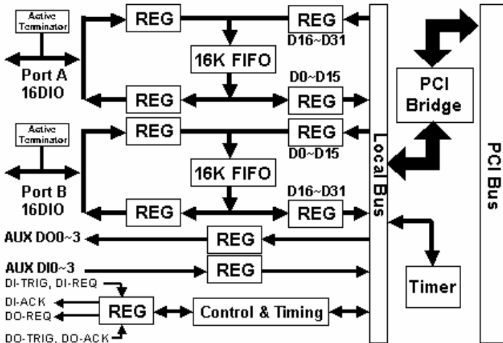
Figure 4.1: Block diagram
