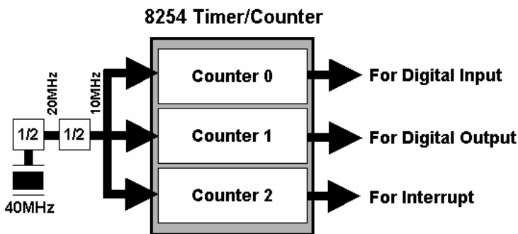
Figure 4.8: Timer configuration
