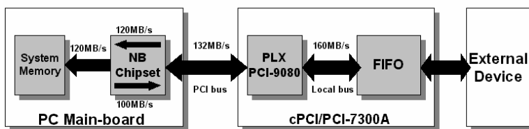
Figure 4.6: Maximum data throughput
